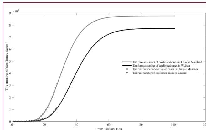
Figure 8: Prediction results of cumulative number of confirmed cases in China and Wuhan.
