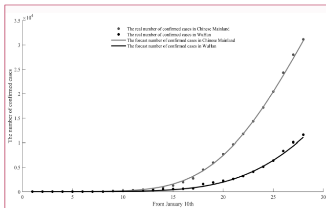
Figure 7: Matching effect chart of the real value and predicted value of the cumulative number of confirmed cases in China and Wuhan.
