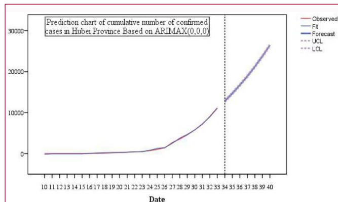
Figure 6: Prediction chart of cumulative number of confirmed cases in Hubei Province Based on ARIMAX (0,0,0).
