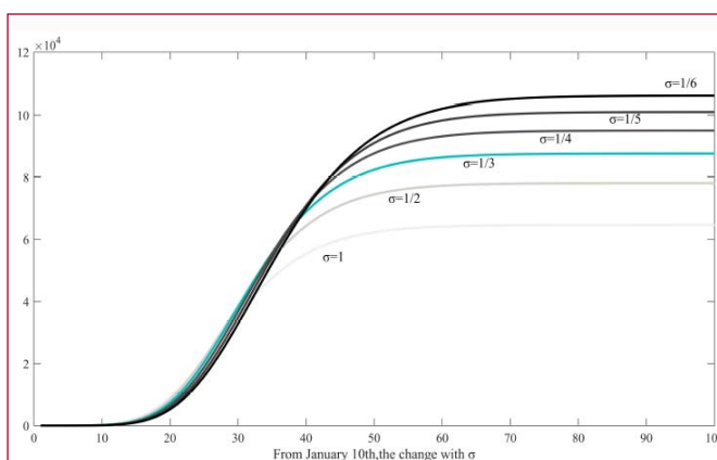
Figure 10: The changes of different \sigma in the cumulative of confirmed cases in mainland China during the COVID-19 transmission process.
