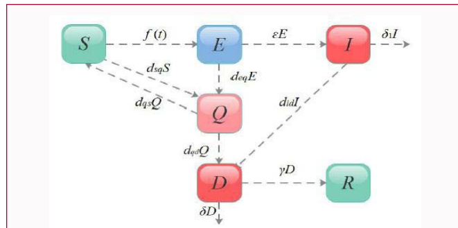
Figure 1: Warehouse transfer diagram of SEIQDR Model.
