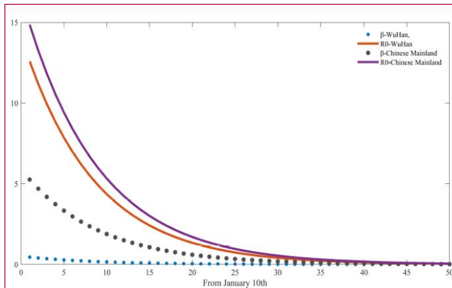
Figure 9: Infection rate \beta and basic regeneration number R_0 in China and Wuhan.
